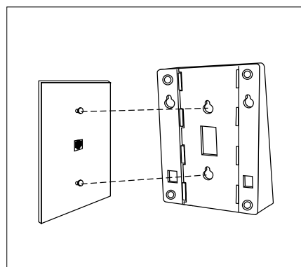
Figure 2-30. Mounting the Stand on the Wallplate
