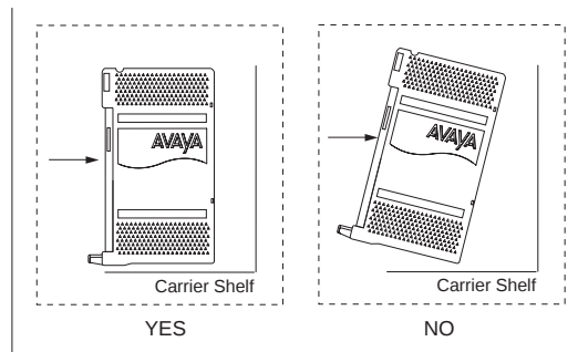
Figure 10-12. Proper Insertion of the Module
