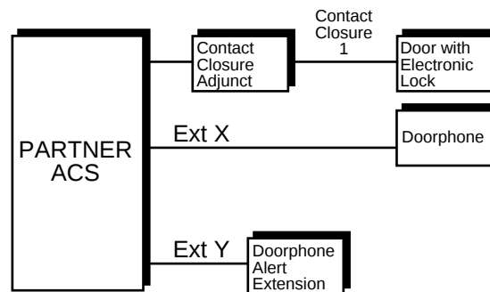
Figure 9-5. Contact Closure Adjunct
