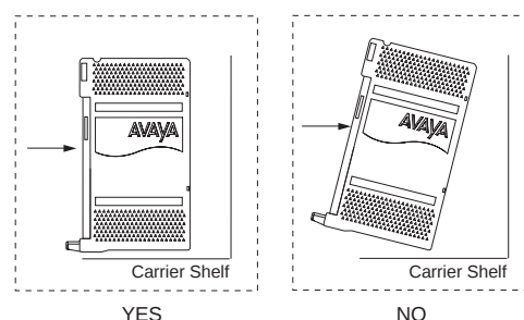
Figure 2-10. Inserting a Module
