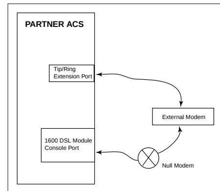
Figure 2-23. Remote Programming Setup
